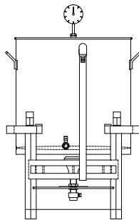
Scalding Tank- Front View
